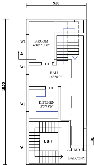
PLAN (FIRST FLOOR) (SCALE 1:100)
