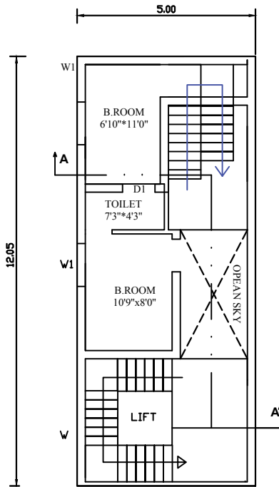
PLAN (SECOND FLOOR) (SCALE 1:100)
