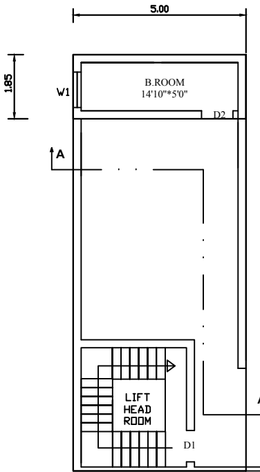
PLAN (THIRD FLOOR) (SCALE 1:100)
