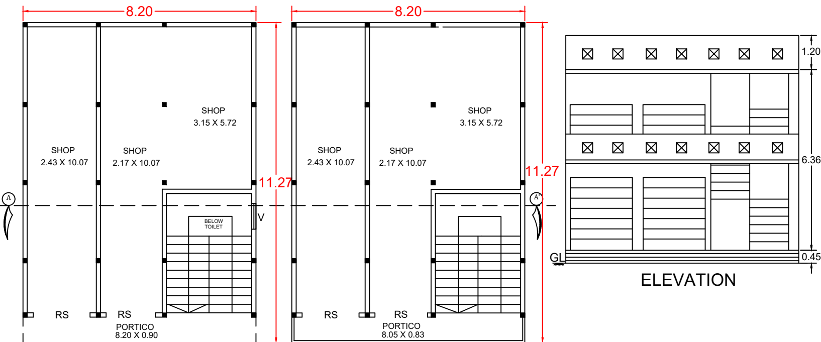
FIRST FLOOR
