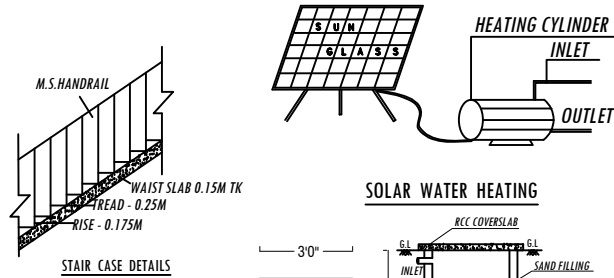
STAIR CASE DETAILS
