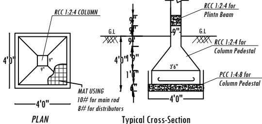
Typical Cross-Section
