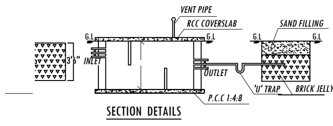
SEPTIC TANK AND DISPERSION TRENCH DETAILS
