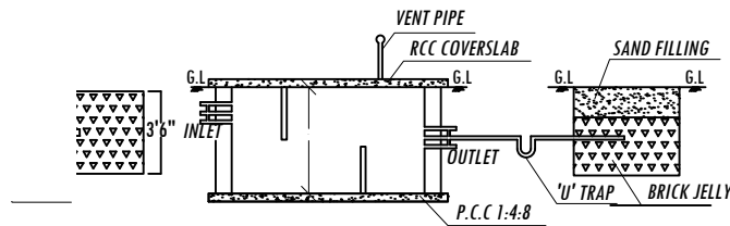
SEPTIC TANK AND DISPERSION TRENCH DETAILS
