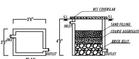
SECTION DETAILS RAINWATER HARVESTING SYSTEM
