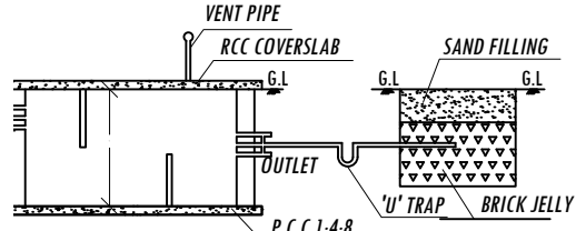
SECTION DETAILS RAINWATER HARVESTING SYSTEM
