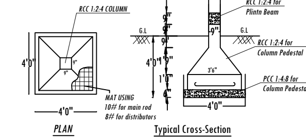
Typical Cross-Section
