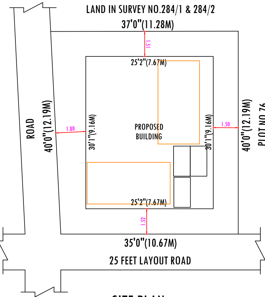
SITE PLAN
