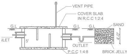
SECTION-AB
