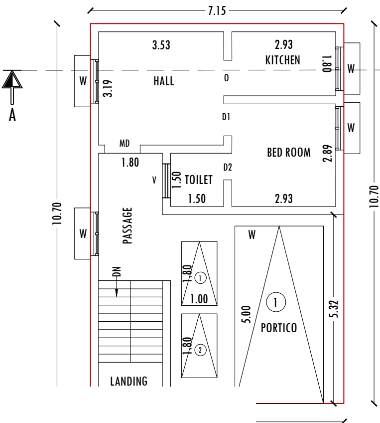
R PLAN
