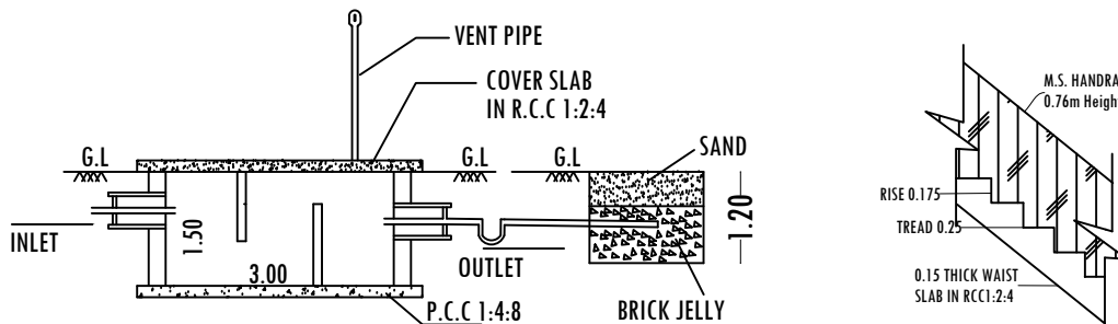
SECTION-AB
