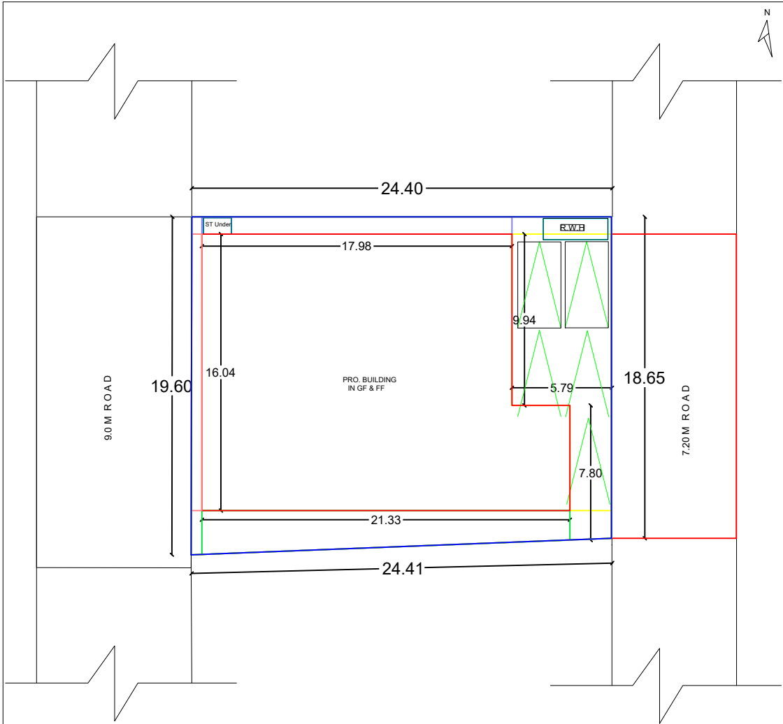
SITE PLAN
