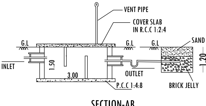
SECTION-AB
