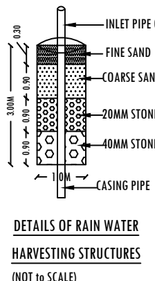
DETAILS OF RAIN WATER HARVESTING STRUCTURES (NOT TO SCALE)
