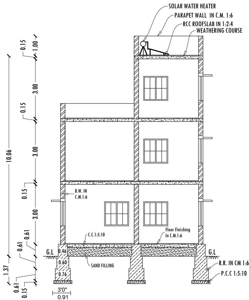
SECTION -AA
