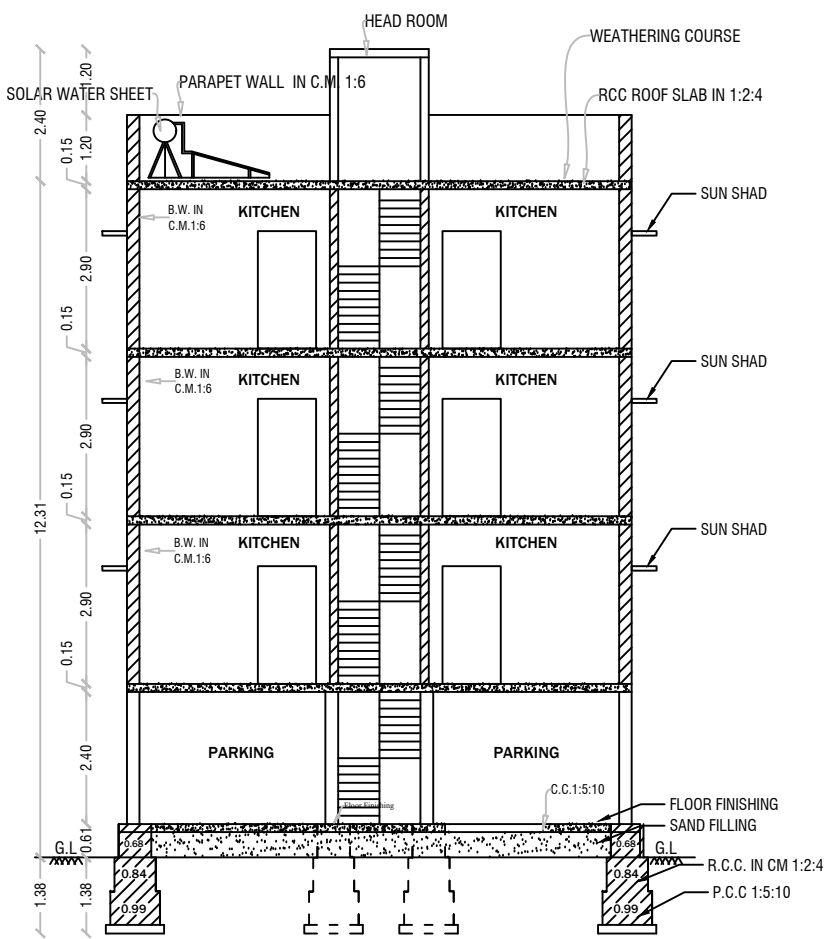
SECTION-AA
