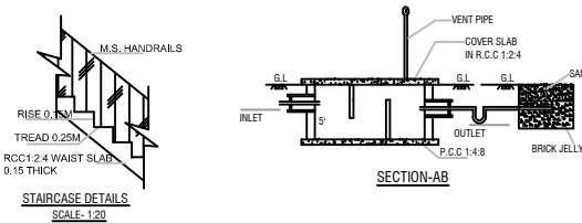
STAIRCASE DETAILS
