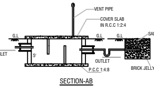
SECTION-AB
