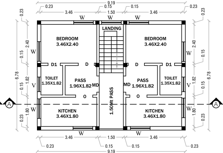
TYPICAL FIRST, SECOND & THIRD FLOOR SCALE - 1:100
