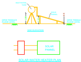
SOLAR WATER HEATER PLAN
