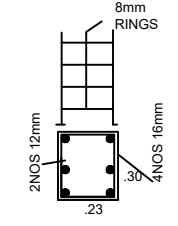
COLUMN DETAILS
