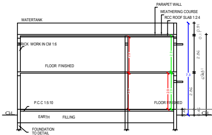
SECTION "A-B"
