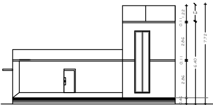
FRONT ELEVATION.
