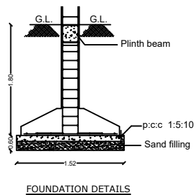
FOUNDATION DETAILS
