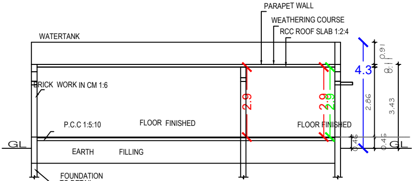
SECTION "A-B"
