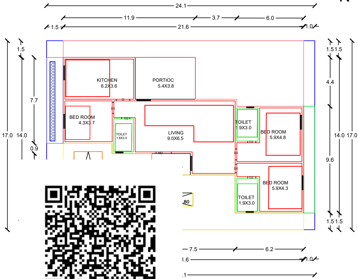
IND FLOOR PLAN.
