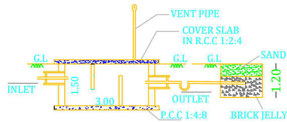
SECTION-AB
