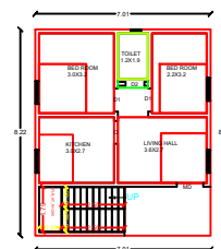
PRO. SECOND FLOOR PLAN.
