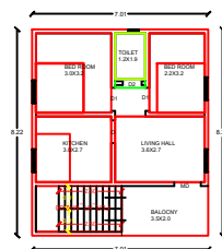
PRO. FIRST FLOOR PLAN.
