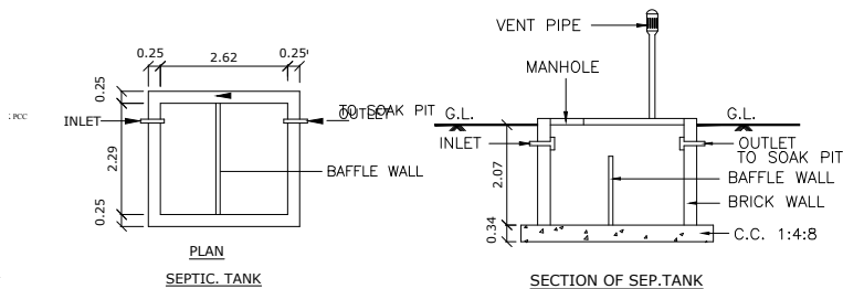
SECTION OF SEP.TANK
