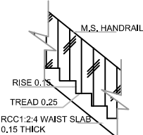
STAIRCASE DETAILS SCALE- 1:20
