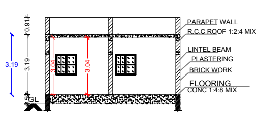
SECTION: A-B
