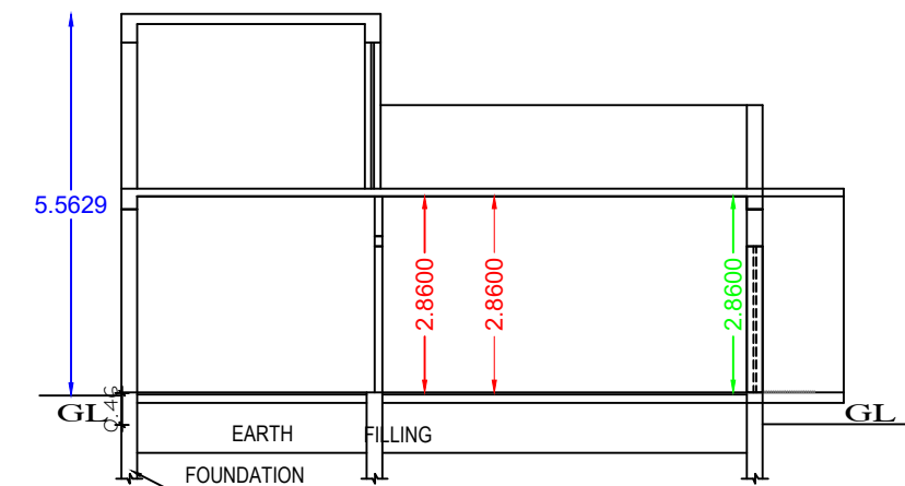
SECTION "A-B"
