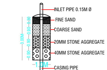
DETAILS OF RAIN WATER HARVESTING STRUCTURES
