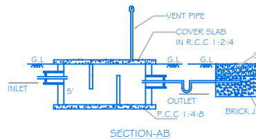
SECTION-AB
