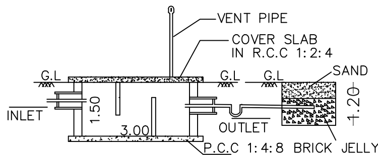
SECTION-AB
