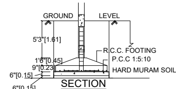
FOUNDATION DETAILS
