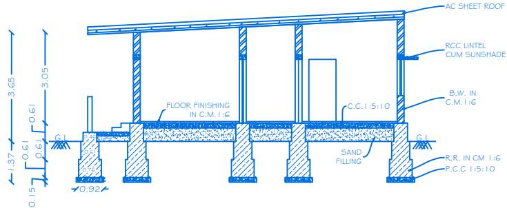
SECTION ON-AA
