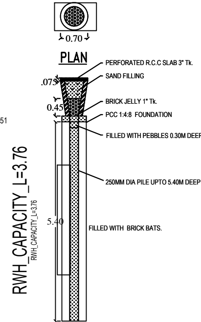
PERCOLATION PIT SECTION OF RAIN WATER
