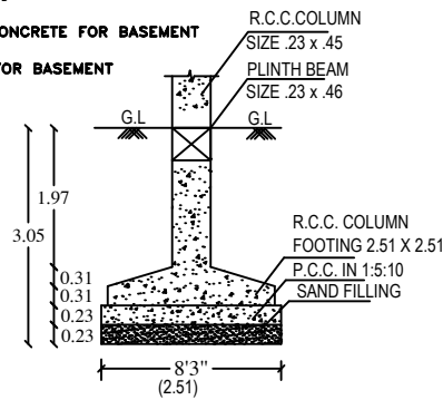
FOUNDATION DETAIL (DETAIL - B)
