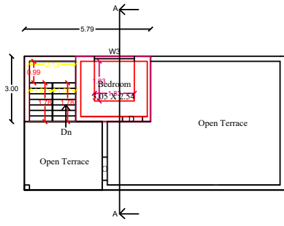
PRO SECOND FLOOR PLAN
