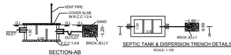
SECTION-AB
