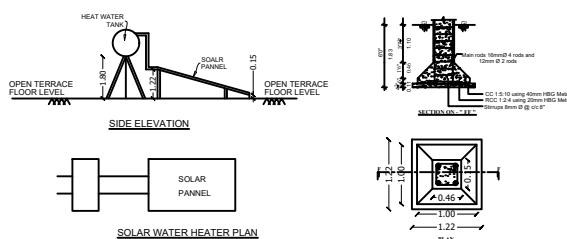
SOLAR WATER HEATER PLAN
