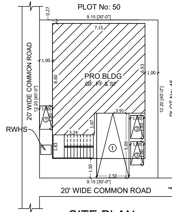
SITE PLAN
