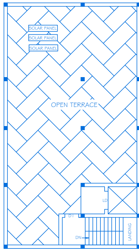
TERRACE FLOOR
