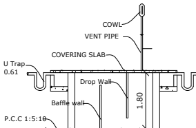
SECTION ON JS
