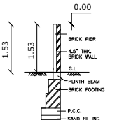
COMPOUND WALL DETAIL
