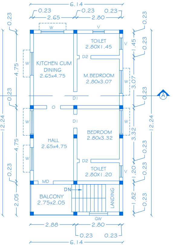
TYPICAL PLAN OF FIRST & SECOND FLOOR
