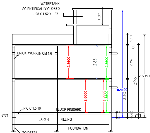
SECTION "A-B"
