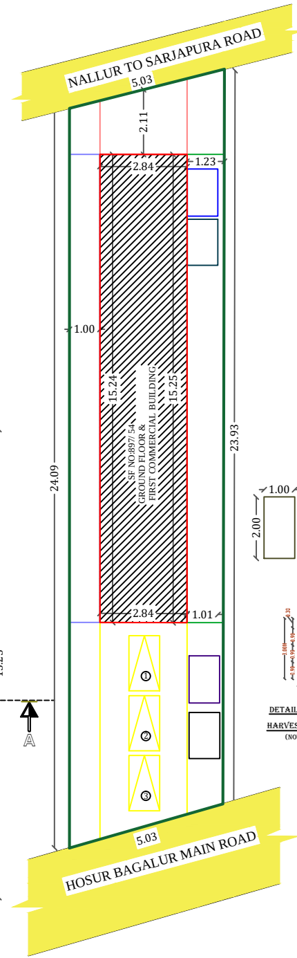
SCALE -1:100
