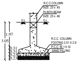
FOUNDATION DETAIL
