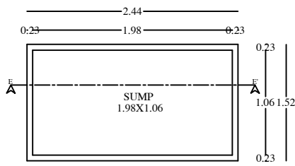
PLAN FOR SUMP
