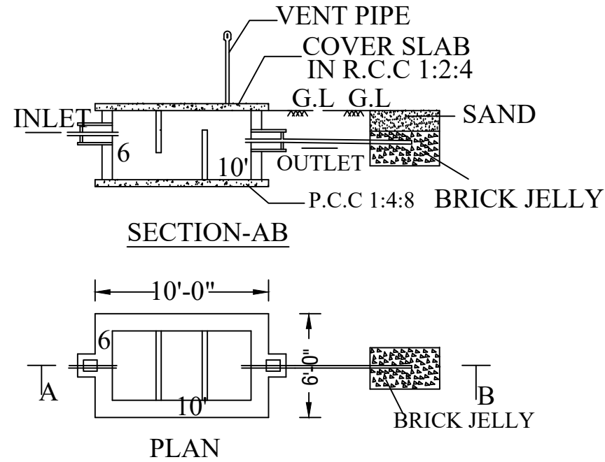
SEPTIC TANK & DISPERSION TRENCH DETAILS SCALE- 1:100
