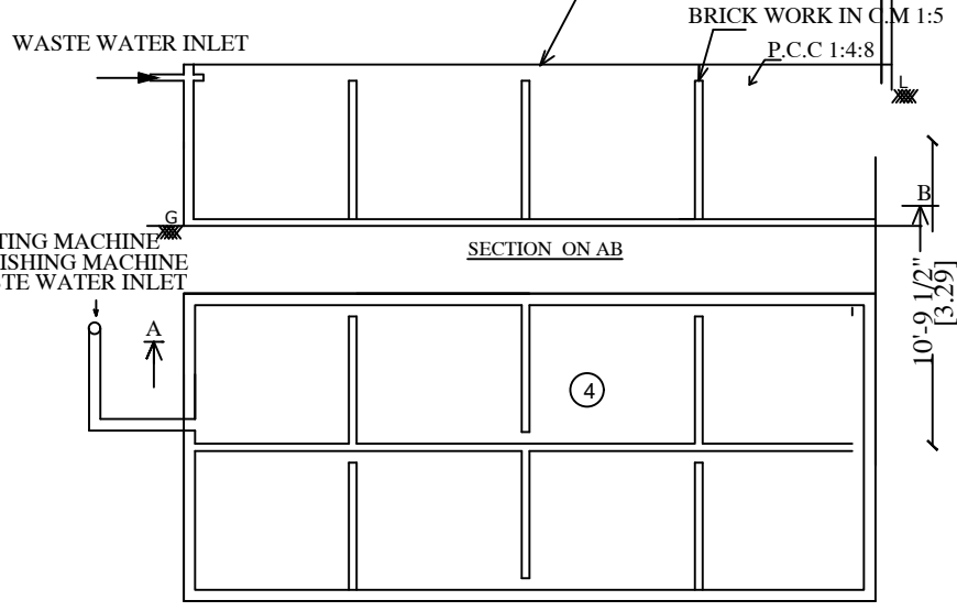
SEWAGE TREATMENT PLANT SCALE- 1:100
