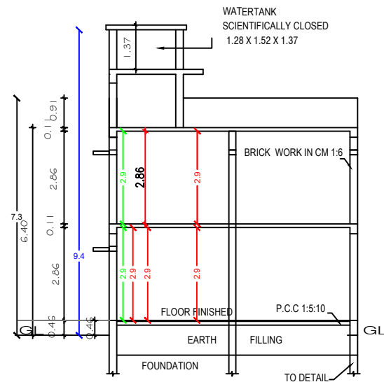
SECTION "A-B"
