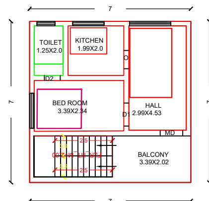
PRO.FIRTS FLOOR PLAN SCALE:1:100
