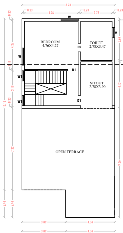
SECOND FLOOR
