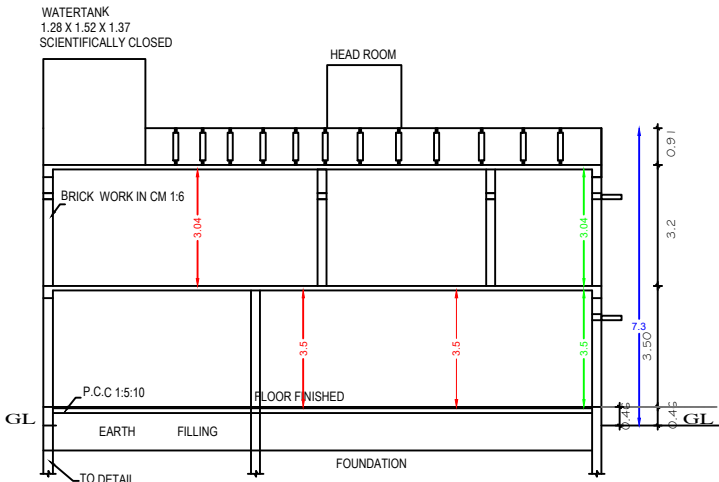
SECTION "A-B"
