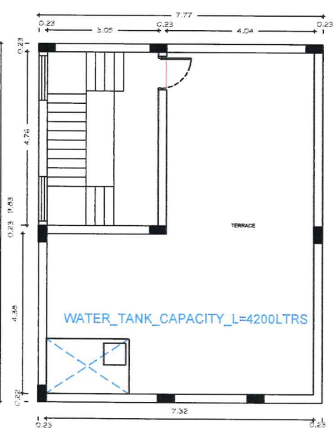
PRO. TERRACE FLOOR PLAN.
