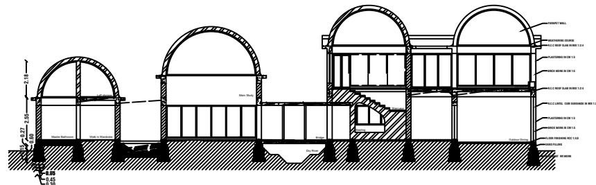
SECTION SCALE 1:100
