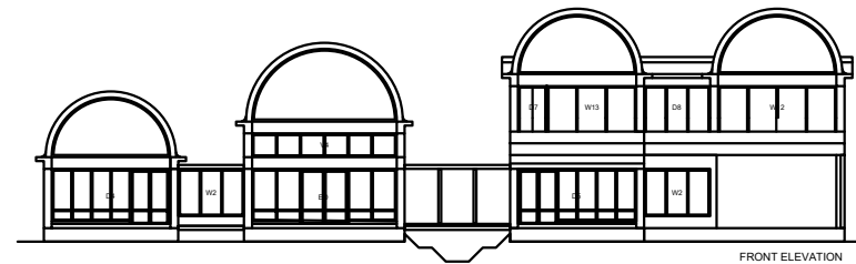
ELEVATION SCALE 1:100
