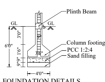
FOUNDATION DETAILS SCALE 1:50
