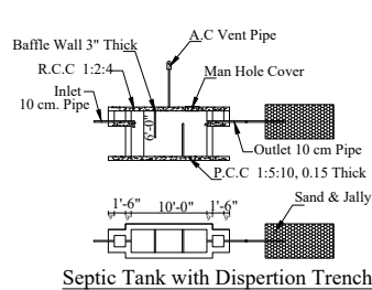
Septic Tank with Dispersion Trench
