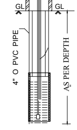
SECTION OF BORE WELL
