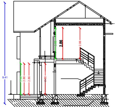
SECTION "A-B"
