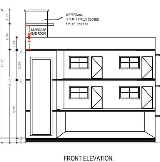
FRONT ELEVATION.
