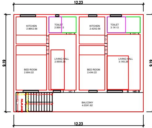
PRO. SECOND FLOOR PLAN.
