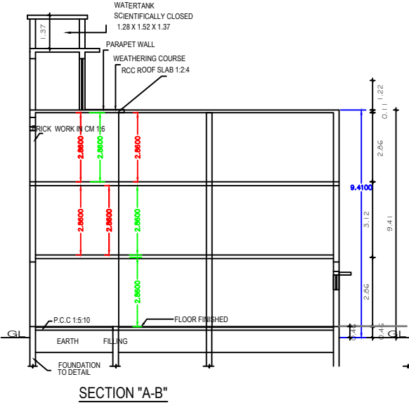
SECTION "A-B"
