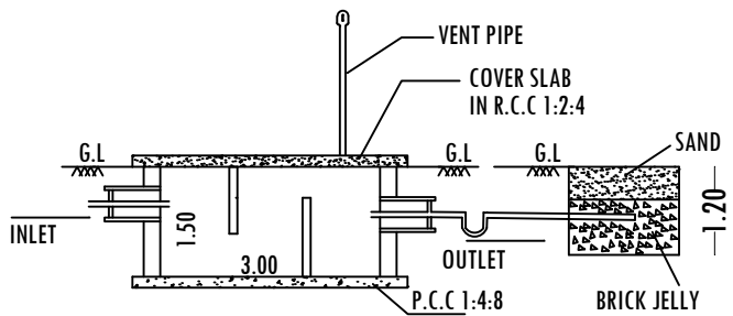
SECTION-AB
