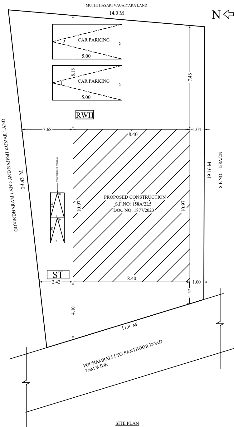
SITE PLAN
