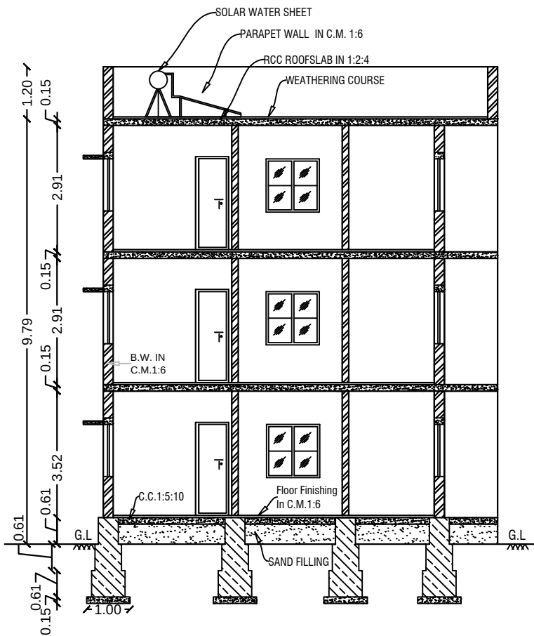
SECTION -AA
