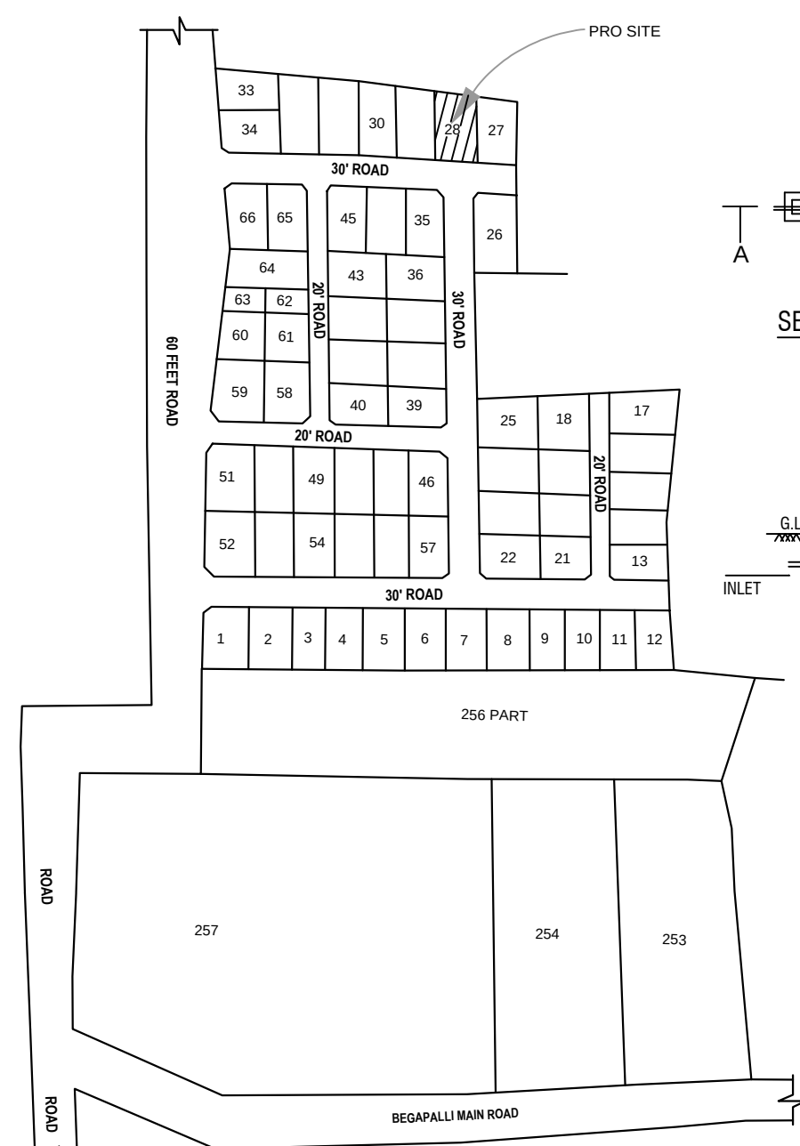
LOCATION PLAN
