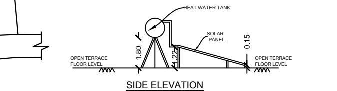
SIDE ELEVATION
