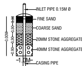
DETAILS OF RAIN WATER
