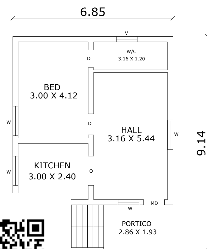
1) FLOOR PLAN
