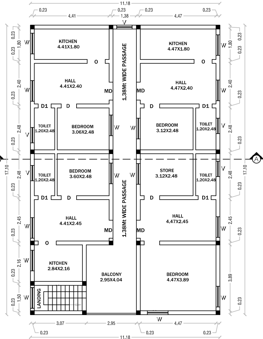
FIRST FLOOR SCALE - 1:100
