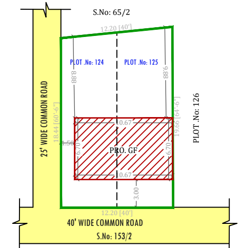
SITE PLAN
